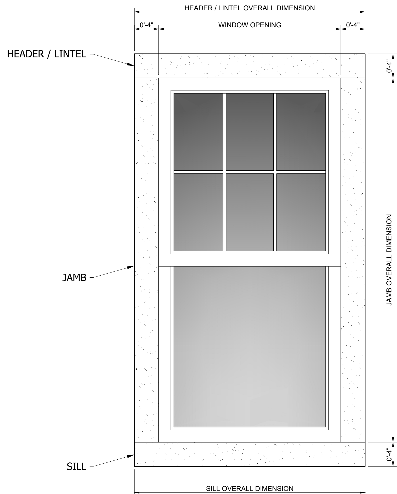
ELEVATION VIEW SCALE 1 1/2"=1'-0"
