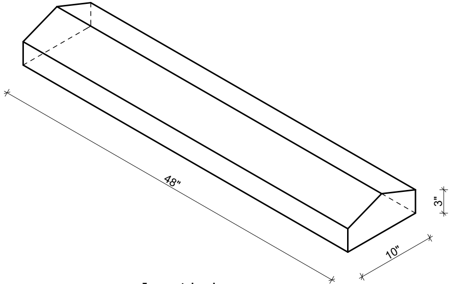
Isometric view
